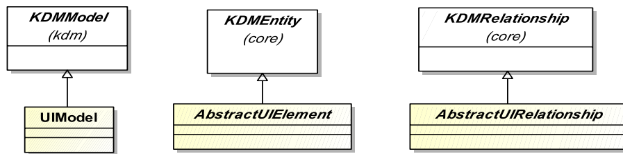
Figure 16.2 - UIInheritances Class Diagram
