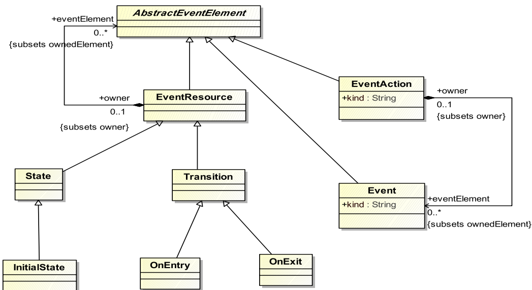
Figure 17.3 - EventResourcesClass Diagram
