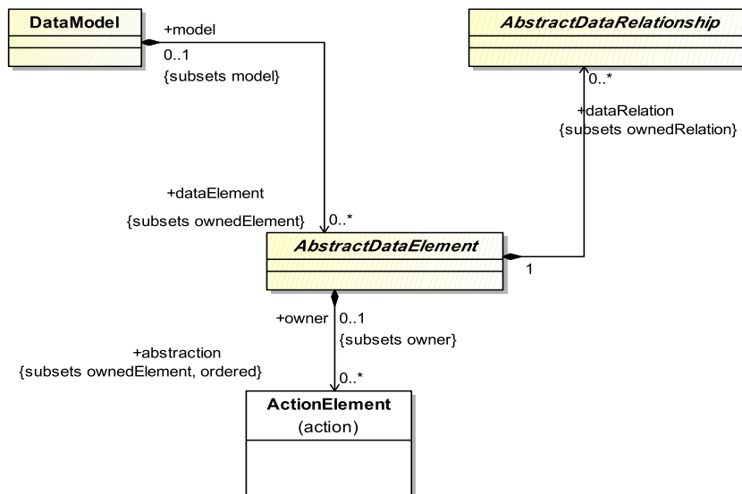
Figure 18.1 - Data Model
