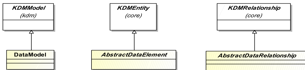
Figure 18.2 - DataInheritances Diagram
