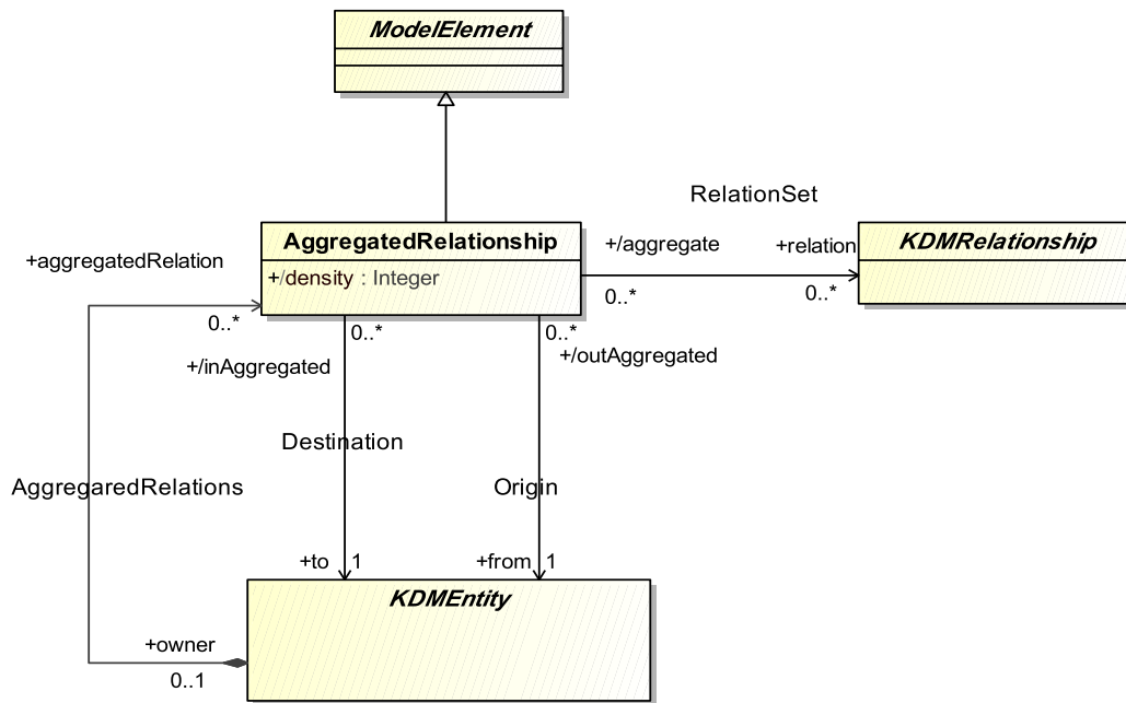
Figure 9.4 - AggregatedRelationships Class Diagram
