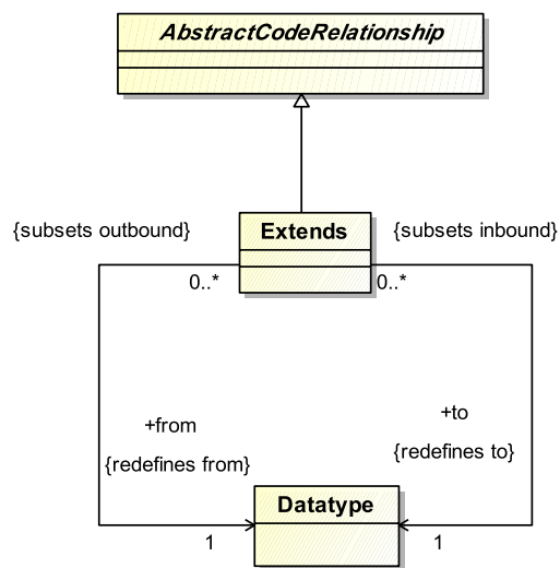
Figure 12.19 - ClassRelations Class Diagram
