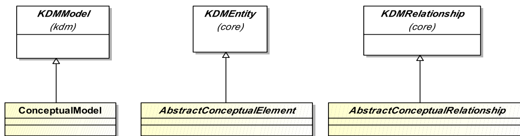
Figure 20.2 - ConceptualInheritances Class Diagram
