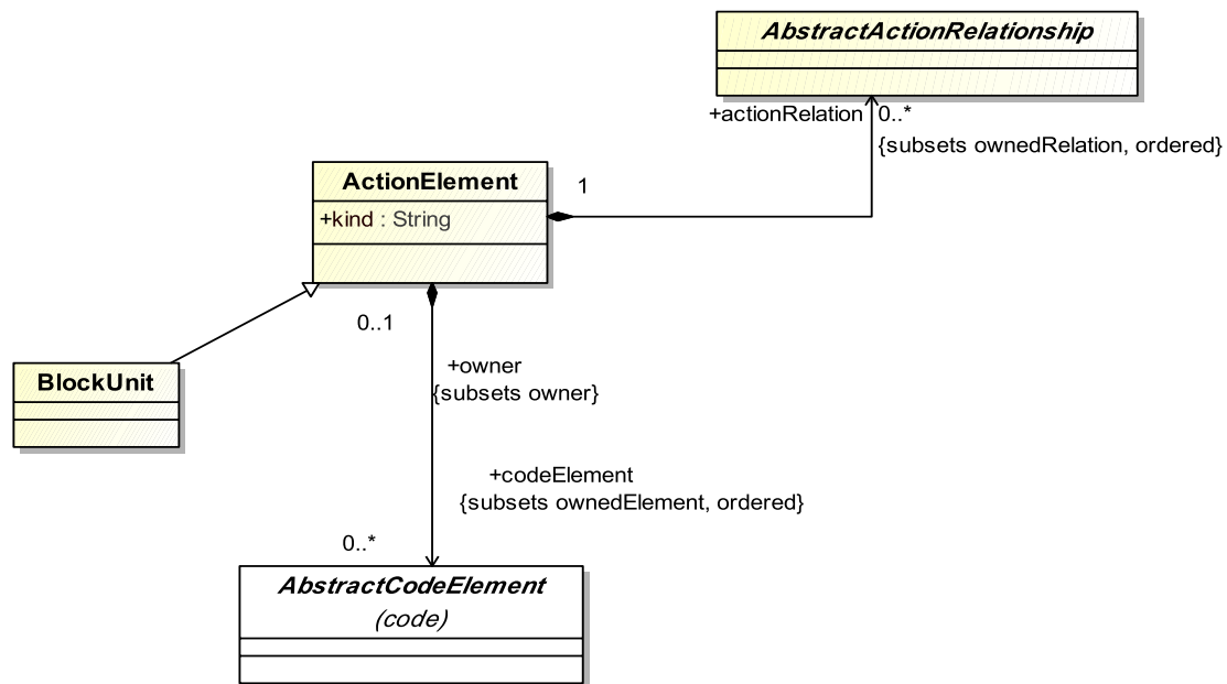
Figure 13.1 - ActionElements Class Diagram
