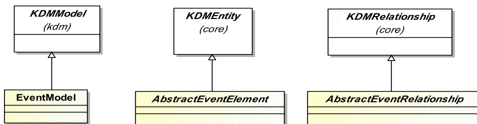
Figure 17.2 - EventInheritances Class Diagram
