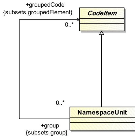
Figure 12.23 - Visibility Class Diagram
