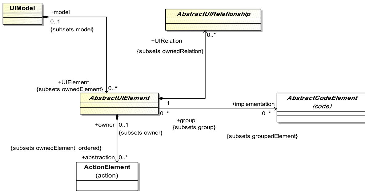
Figure 16.1 - UIModel Class Diagram
