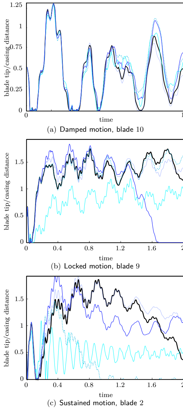
Figure 4 – Convergence of the results obtained with CB method for each kind of interaction \eta = 0 (—); \eta = 44 (---); \eta = 88 (—); \eta = 220 (....); u_{fe}(t) (—)
