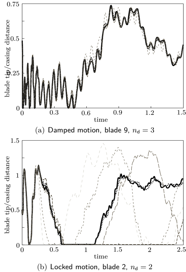
Figure 3 – Blade tip/casing distance for two blades and two different simulations when time steps varies: h = 10^{-5} s (—), h = 5 \cdot 10^{-6} s (—), h = 10^{-6} s (—), h = 5 \cdot 10^{-7} s (—), h = 2.5 \cdot 10^{-7} s (.....) and h = 10^{-7} s (—)
