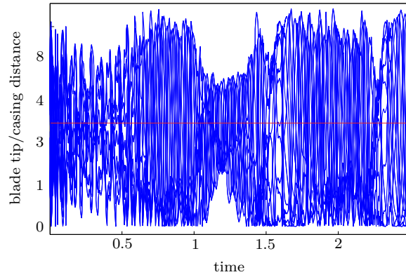
(b) Sustained motion: \Omega = 1.75 , n_d = 3
