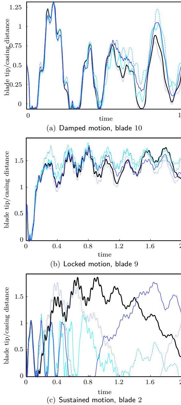
Figure 5 – Convergence of the results obtained with CCM method for each kind of interaction \phi = 0 (—); \phi = 44 (---); \phi = 88 (—); \phi = 220 (....); u_{fe}(t) (—)
