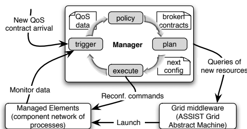
Figure 7: ASSIST framework.
