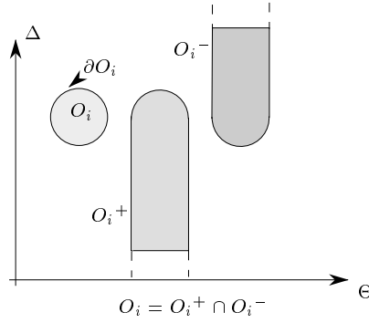
FIG. 2.2 – Defining O_i^+ and O_i^- .
