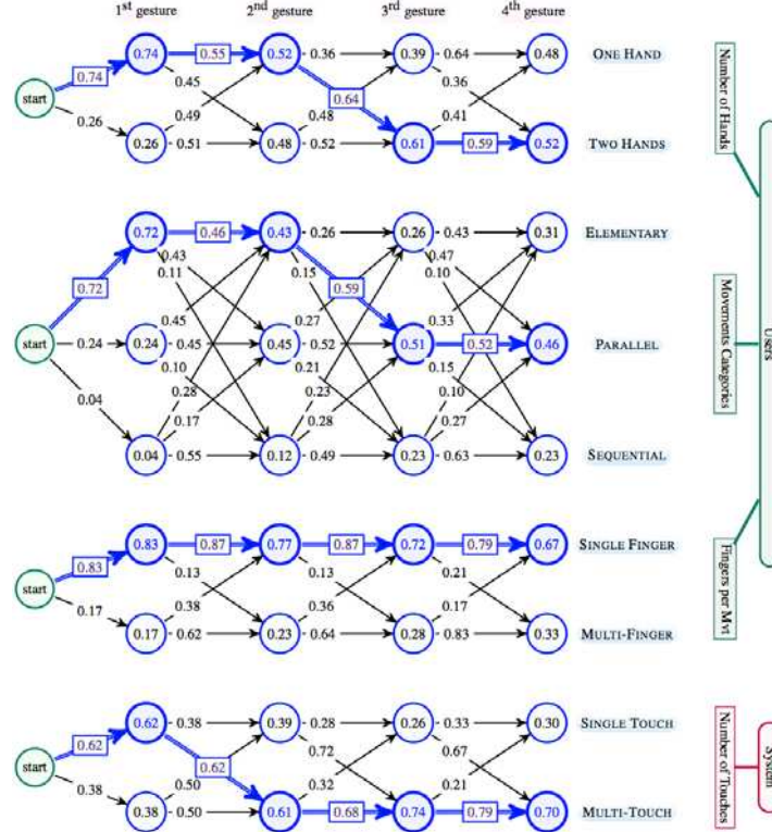
Fig. 6. Gestures Transition-Frequency Automaton (average over all symbols and users) according to (from top to bottom): Number of Hands, Movement categories, Number of fingers per atomic movement, and Number of contacts.
