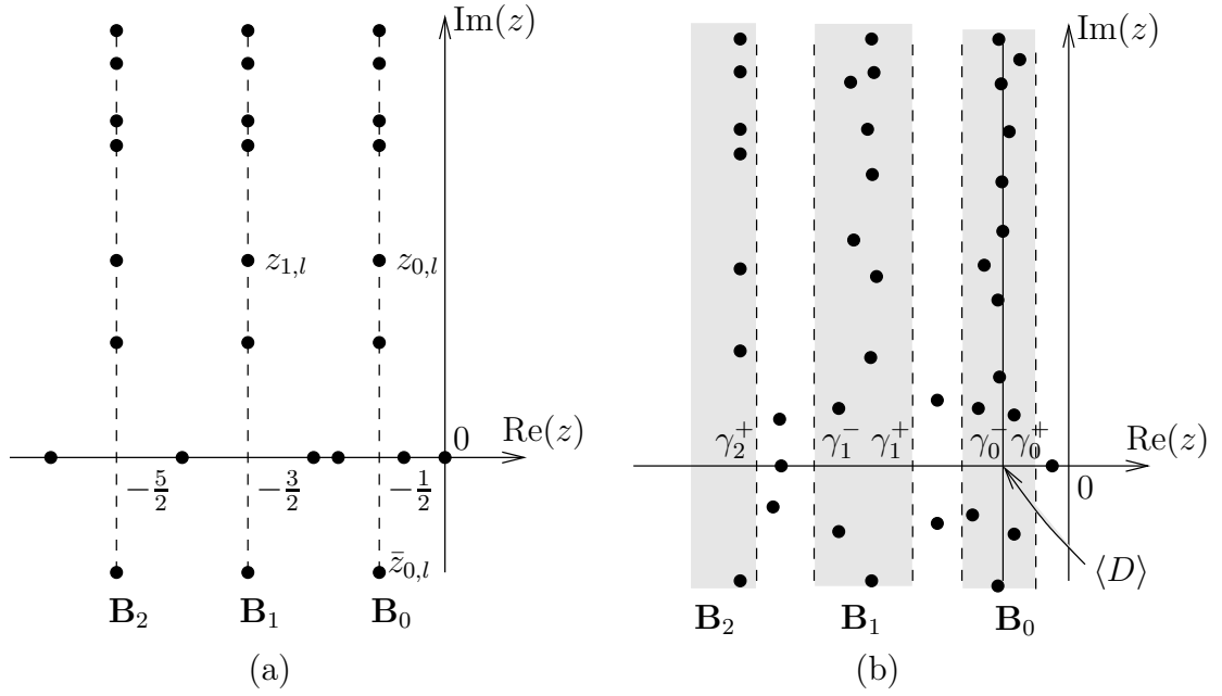
Figure 5.1: (a) For an hyperbolic surface \mathcal{S} = \Gamma \backslash \mathbb{H}^2 , the Ruelle-Pollicott spectrum of the geodesic vector field -X given by Proposition 4.1. It is related to the eigenvalues of the Laplacian by (4.1). (b) For a general contact Anosov flow, the spectrum of A = -X + V and its asymptotic band structure given by Theorems 5.1 and 5.3.
