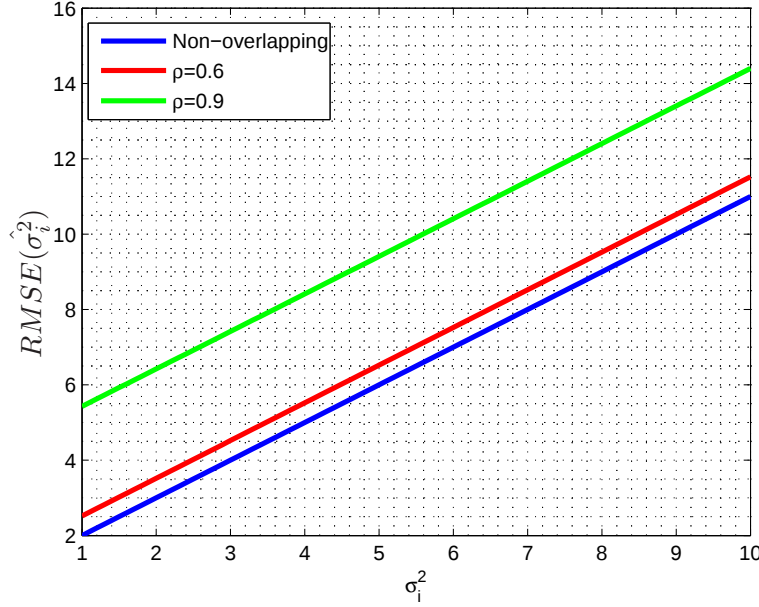
Figure 3.7: RMSE of \hat{\sigma}_i^2 as a function of \sigma_i^2 for W = 1 MHz, \sigma_j^2 = 20 .
