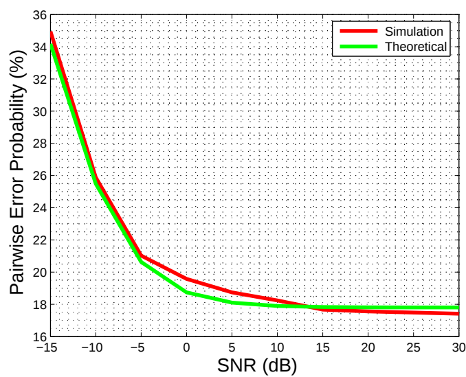
Figure C.19: PEP pour \beta = 1.1 .
