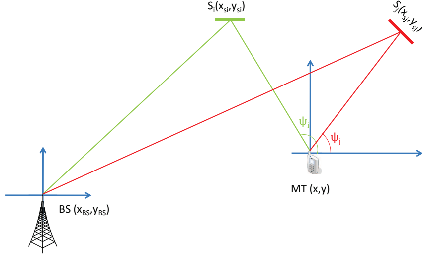
Figure 3.8: BS-MT geometry.
