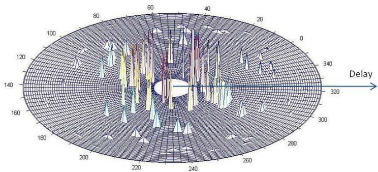
Figure C.4: Power Delay Angle of Arrival Profile
