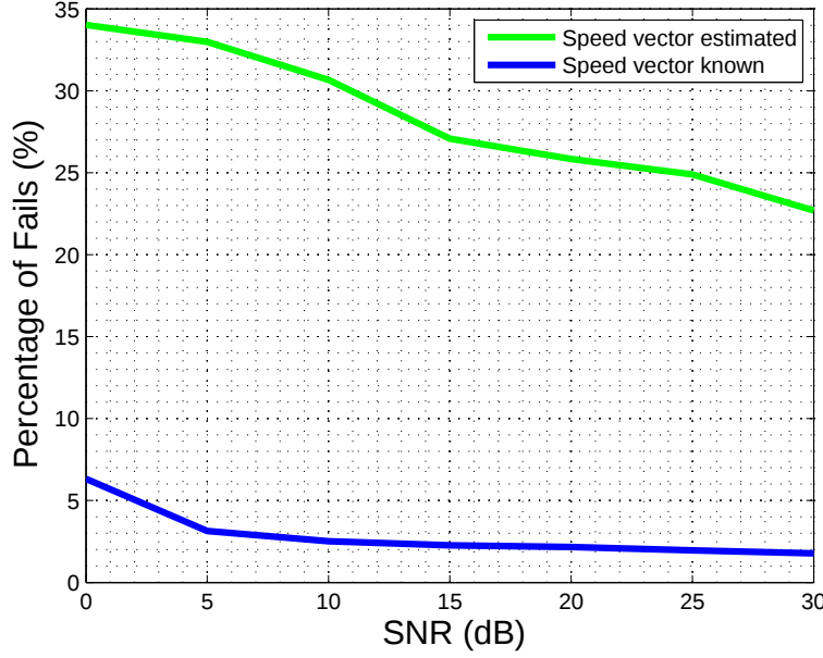
Figure 2.7: Time domain PDDP-F for n = 2 with and without speed vector estimation.
