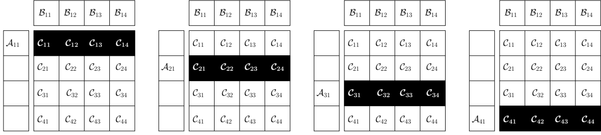
Figure 4.7: Four steps of the maximum re-use algorithm, with m = 21 and \mu = 4 . Updated elements of C are written white on black.
