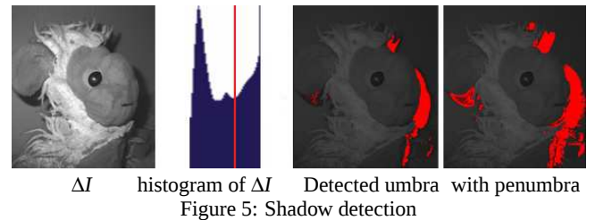
Figure 5: Shadow detection
