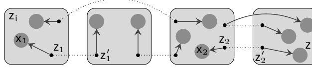
Figure 5: Zones and wires of a graph.
