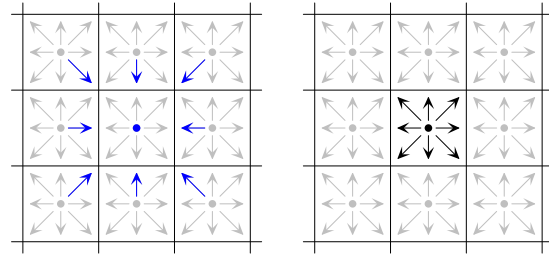
Figure 5: Out-of-place propagation
