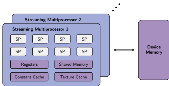
Figure 2: CUDA hardware
