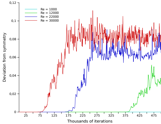
Figure 12: Evolution of \mathcal{L} at different Reynolds numbers
