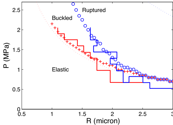
FIG. 7. Phase diagram of the different oscillation behaviour. Thick lines: experimentally measured on polymer contrast agents 9 boundaries for onset of transient zone (first thick line when increasing pressure) and onset of immediate rupture (second thick line). Symbols: numerical prediction, the shell parameters being adjusted to fit the measured boundaries, with the onset of buckling (crosses) and the onset of rupture (circles). The static buckling pressure 2\sigma_m^{buckling}/R_0 (first dotted line when increasing pressure) provides a good approximation of buckling, while the static rupture pressure (second dotted line) is overestimating the dynamical value. Shell parameters are \chi_{2D} = 10 N/m, \kappa_s = 7.2 \times 10^{-9} N, while the buckling tension is \sigma_m^{buckling} = -1 N/m, and the rupture tension is \sigma_m^{break-up} = 3.5 N/m, under an ultrasound frequency of f = 1.7 MHz.
