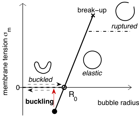
FIG. 4. Model for the shell membrane tension under large volume variation. As soon as the surface tension is negative enough to reach the buckling value (full circle), buckling occurs (large arrow) and the membrane tension vanishes (thick dashed line). The elastic state is recovered when the volume gets back to its rest value (open circle). When the rupture point is reached (cross), membrane tension saturates to the water value (dash dotted).
