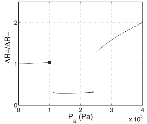
FIG. 6. Effect of an increasing acoustic pressure on the asymmetry of the response. Same shell parameters as in figure 5.
