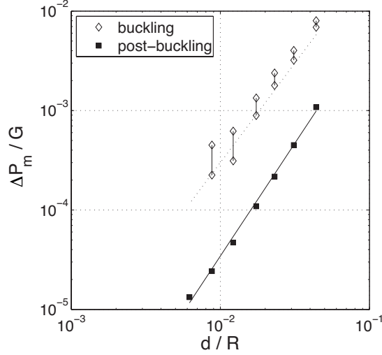
FIG. 2. Simulation results for the post-buckling pressure \Delta P_m^{\text{post-buckling}} (squares), evaluated in the plateau region of Fig. 1d, as a function of the relative shell thickness. The continuous line stands for a power-law fit with \Delta P_m^{\text{post-buckling}}/G = 1.193 \times (d/R)^{2.27 \pm 0.06} . The value of the exponent is in total agreement with theoretical predictions of post-buckling pressure derived in Appendix B. For comparison, we also plot the buckling pressure \Delta P_m^b from simulations (diamonds giving the range where simulation value is located), and the theoretical prediction (dashed line) from Eq. 7.
