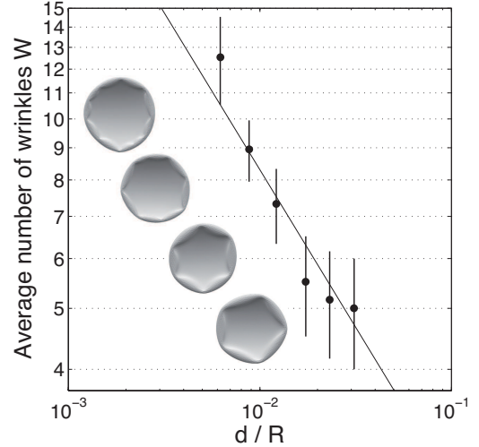
FIG. 3. Simulation of the number of wrinkles hold by the single depression of a deflating elastic spherical surface, as a function of the relative shell thickness for a thin shell of incompressible material. This number is an average for important deflations, i.e. when the size of the depression approaches one hemisphere, and before autocontact ; practically we averaged for \Delta V/V \in [0.53, 0.76] . Points are dispersed but compatible with the power-law in (d/R)^{-1/2} observed in 26 . Here the line is a fit with Eq. 8. Inserted snapshots are taken from simulations of shells with 10, 8, 6 and 5 wrinkles, from left to right.
