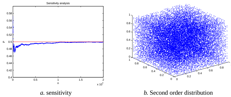
Fig. 1. Security analysis
