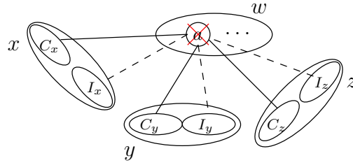
Fig. 2. A failed value (w, a) , its compatible values in C_x , C_y and C_z and its incompatible values in I_x , I_y and I_z .
