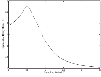
Fig. 1: Bound on Decay Rate vs. Synchronous Sampling Period, T_{\min} = T_{\max} for Example 2 with N = 3 .
