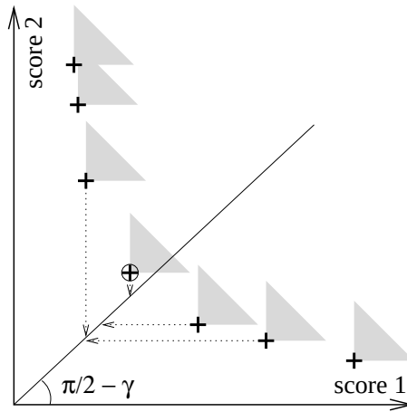
Fig. 3 Conc \beta -selection visual description. N.B. In that case only, score_1 and score_2 have to be minimized.
