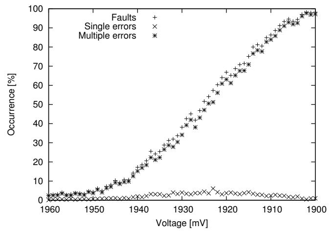
Figure 7b. Occurrence of fault — WDDL.
