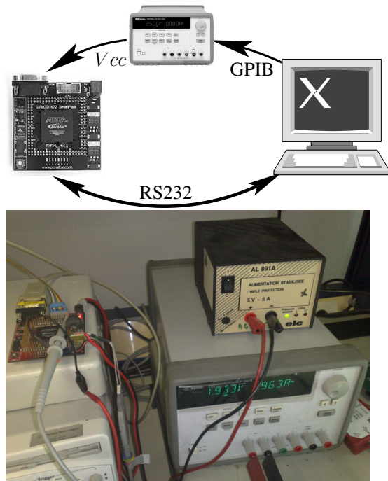
Figure 6. Experimental platform.
