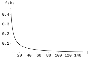
FIGURE 3. f(k) - k + 1 > 0 .
