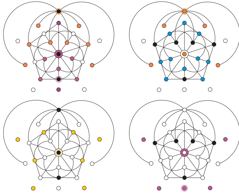
Figure 1: A pictorial illustration of the structure of the Veldkamp lines of \mathcal{V}(\text{GQ}(2,4)) . Left : – A line of Type I, comprising three distinct perps (distinguished by three different colours) having collinear centers (encircled). Right : – A line of Type II, featuring two perps with non-collinear centers (orange and purple) and a doily (blue). In both the cases the black bullets represent the common elements of the three hyperplanes.
