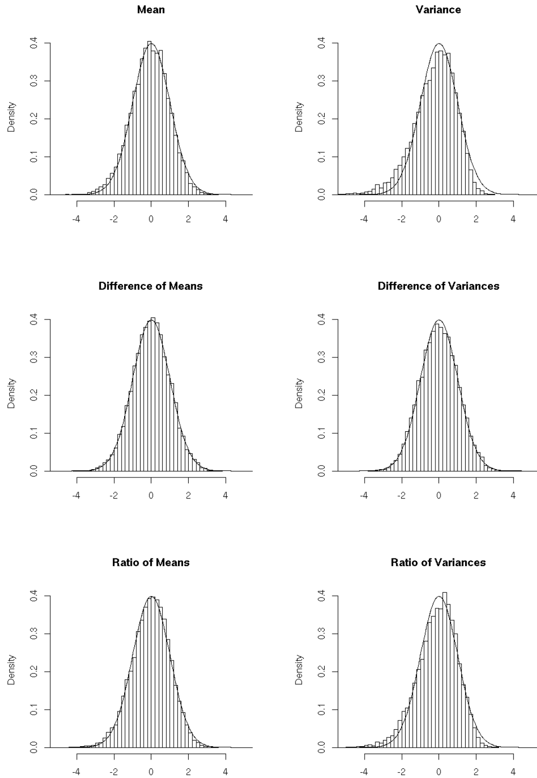
Figure 3: Histograms of m = 10000 replications of \frac{\hat{\theta}(\mathbf{Y}) - \theta}{\hat{\sigma}_{\hat{\theta}}(\mathbf{Y})} for \theta = \mu, \sigma^2, d_\mu, d_{\sigma^2}, r_\mu and r_{\sigma^2} . The simulation has been done as follows: n = n^{(1)} = n^{(2)} = 500 , Y^{(1)} \rightsquigarrow \mathcal{E}(1) , Y^{(2)} \rightsquigarrow \mathcal{E}(1) .
