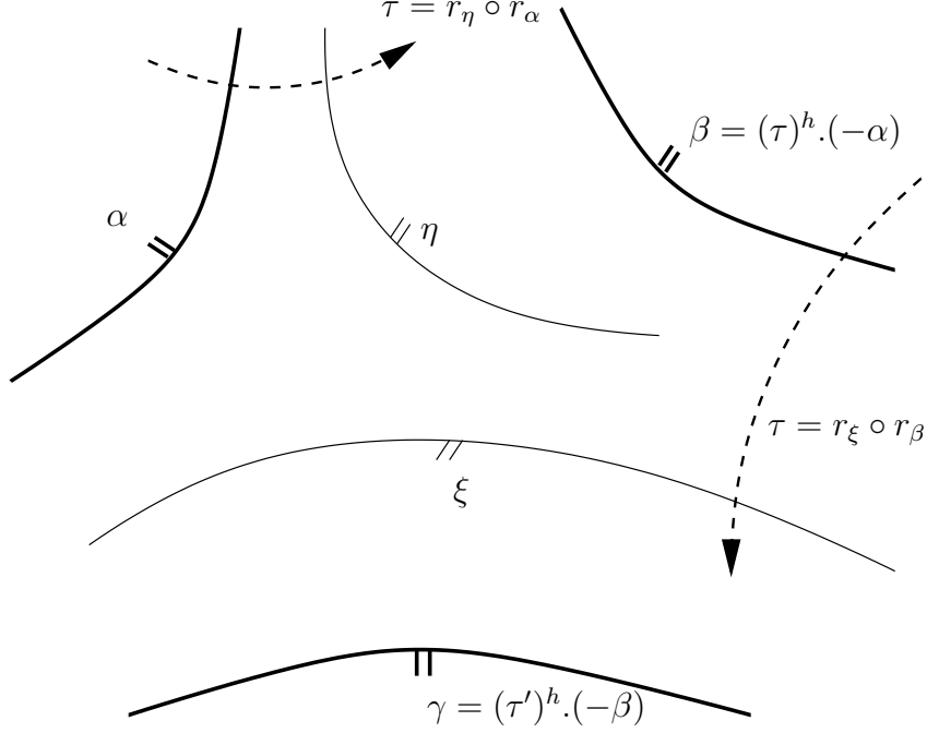
FIGURE 1. Proof of Theorem 15
