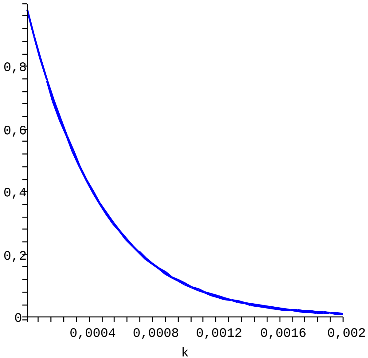
Figure 4: M (the mass at W_{max} ) function of the drop probability k for W_{max} = 64 .
