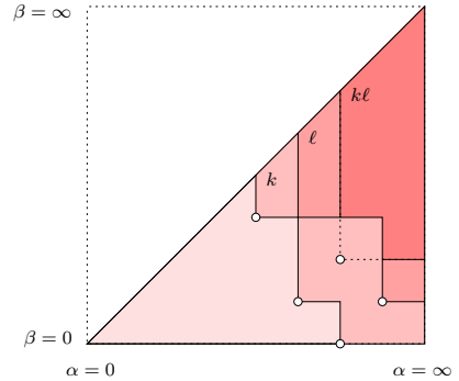
Fig. 2. Since vertices have no proper faces, Q(k, X) and Q(\ell, X) are unions of quadrants. For the edge, Q(k\ell, X) is the portion of its union of quadrants inside Q(k, X) and Q(\ell, X) .
