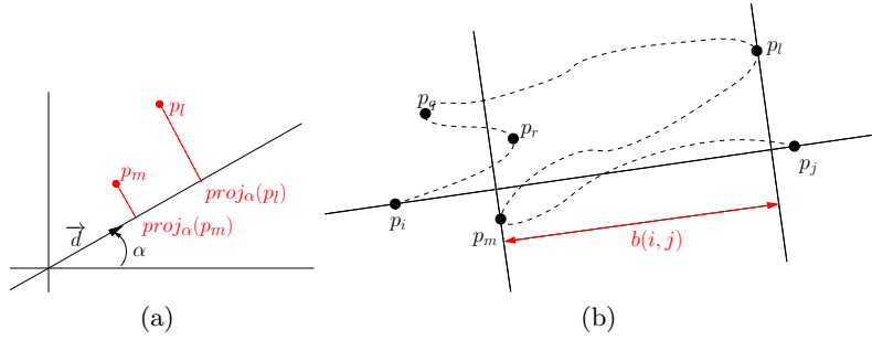
Fig. 1. (a) Illustration of Definitions 1 and 2. (b) Illustration of backpaths in direction \vec{p_i p_j} : \vec{p_r p_q} is a backpath since it is a negative shift and p_r is before p_q on the curve P(i, j) . However, it is not the longest backpath: \vec{p_l p_m} is also a backpath, of maximal length b(i, j) .
