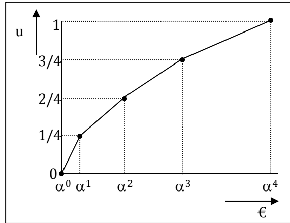
Figure 2.3.1. Utility graph derived from \sim^* observations
