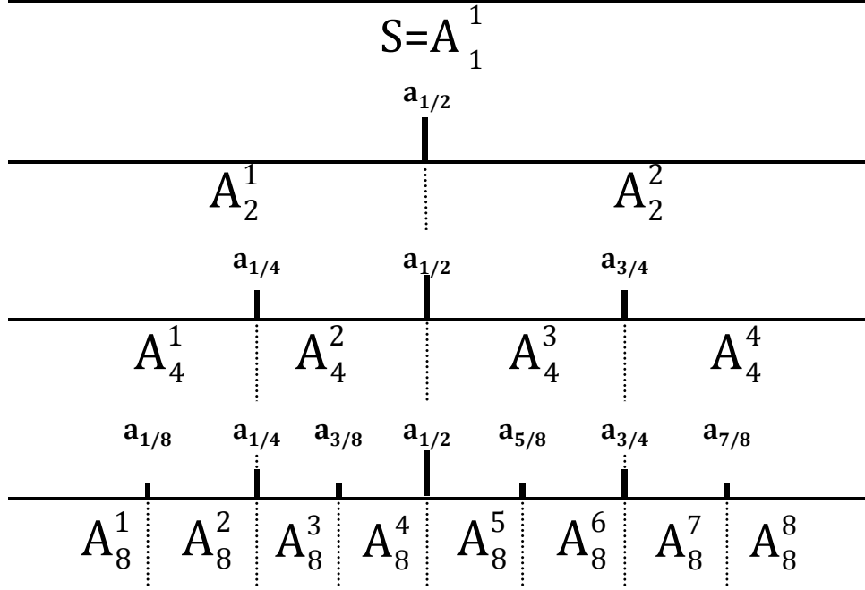
Figure 5.3.1: Decomposition of the state space
