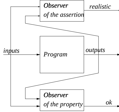
Figure 1: Verification program
