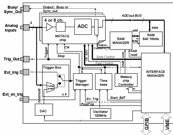
Fig. 4: Synopsis of the MATAcqVME board.
