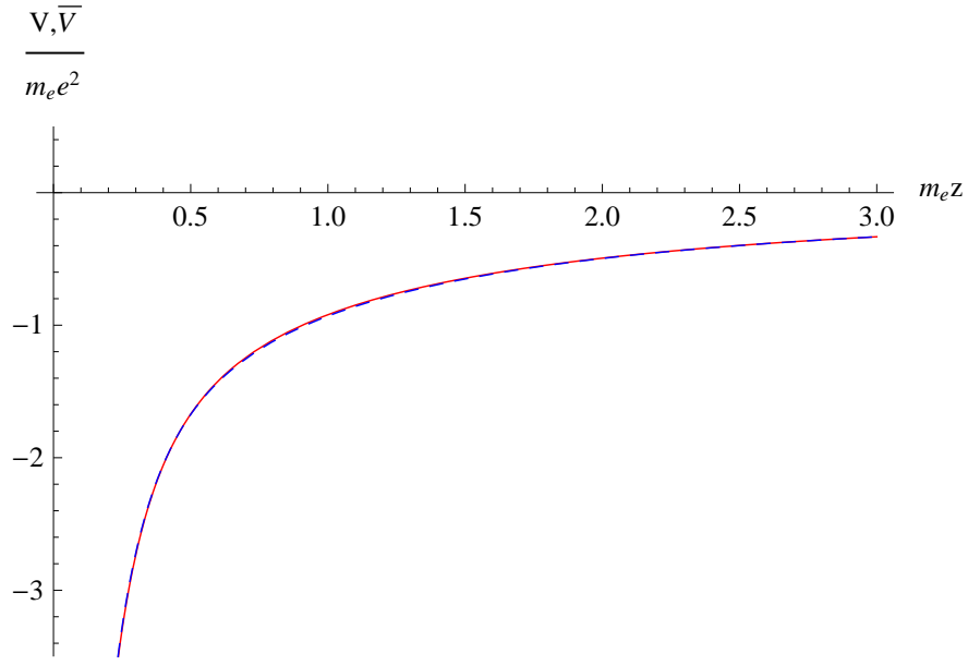
Fig. 5. Modified Coulomb potential energy at B = 10^{17} \text{ G} . Analytical formula (approximate \bar{P} ) in blue-dashed versus numerical integration (exact P ) in red (the two curves practically coincide).
