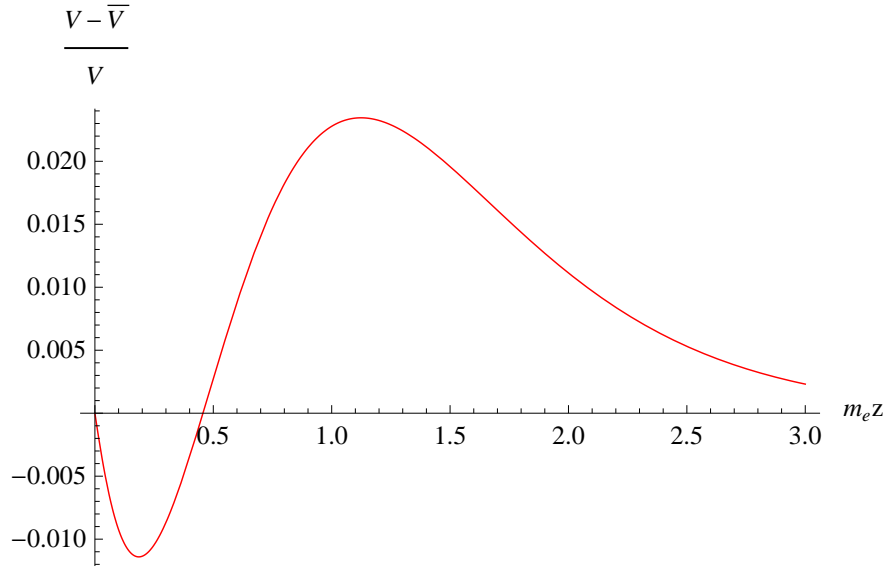
Fig. 6. Relative accuracy of the analytical formula for the modified Coulomb potential energy at B = 10^{17} \text{ G} .
