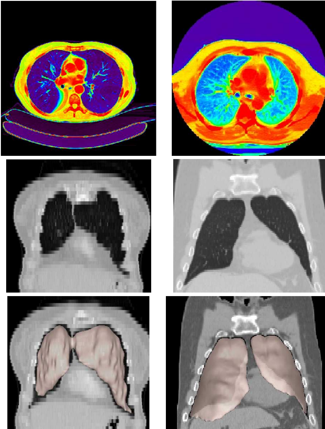
Figure 4.6: Ambiguities solved by consistency verification checks. Top: Presence or absence of a circle limiting the FOV of the CT image. Middle and bottom: low (left) and high (right) resolution CT images with joint (left) or separated (right) lungs, leading to the selection of one or two connected components in the segmentation procedure. The 3D rendered segmented lungs are shown in the bottom images.
