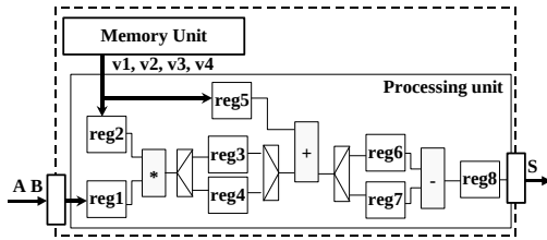
Fig. 2: Sequential architecture
