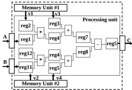
Fig. 3: Parallel architecture
