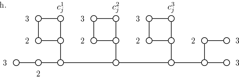
Figure 1: Graph F(C_j) representing a clause C_j of size 3.
