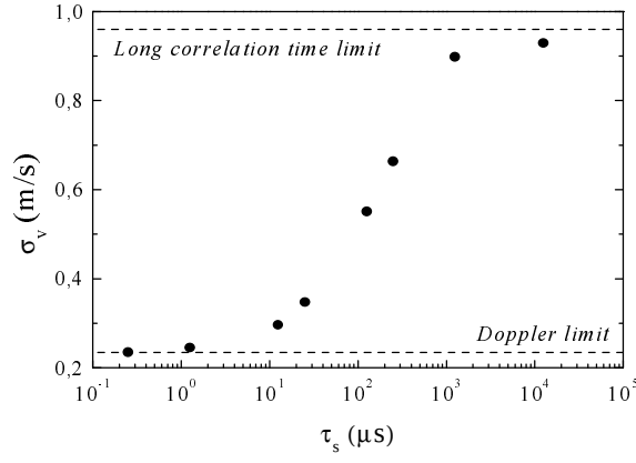
FIG. 7: Final velocity dispersion \sigma_v as a function of the correlation time \tau_s (full circles). The transverse and longitudinal velocity dispersions are both equal to \Delta v = 0.8 \text{ m/s} . The mean saturation of each beam is s_0 = 0.04 and the saturation fluctuation parameter is r_s = 9\% . The upper dashed line represents the long correlation time limit while the lower one represents the Doppler-cooling limit (see text).
