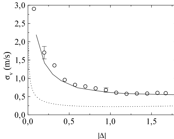
FIG. 3: Velocity dispersion \sigma_v as a function of |\Delta| = 2|\delta|/\Gamma for s_0 = I/I_s = 0.08 . The experimental data (circles) are compared to the Doppler prediction (dotted line) and to the Monte-Carlo simulation (solid line) at r_s = 9\% and \xi_s = 60 \mu m . As one can see the Doppler theory is completely off while very good agreement is obtained with our theoretical model (see text).
