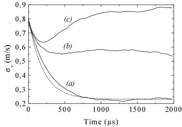
FIG. 9: Monte-Carlo simulations of the time evolution of the velocity dispersion \sigma_v for three characteristic correlation times: (a) short correlation time ( \tau_s = 1.25 \mu\text{s} ) ; (b) intermediate correlation time ( \tau_s = 125 \mu\text{s} ) ; (c) long correlation time ( \tau_s = 1250 \mu\text{s} ). The transverse velocity dispersion is \Delta v_{\perp} = 0.8 \text{ m/s} , the mean saturation per beam is s_0 = 0.04 and the saturation fluctuation parameter is r_s = 9\% . The dashed exponential decay is the bare Doppler prediction (see text).
