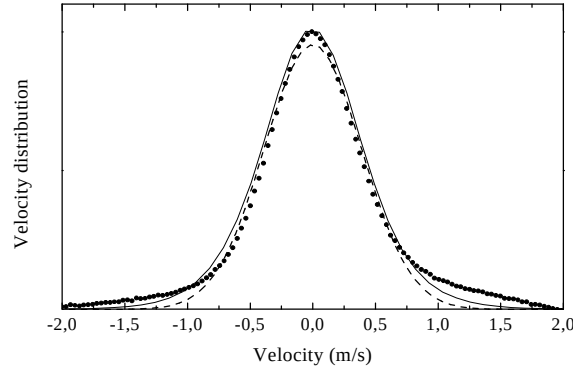
FIG. 8: Velocity distribution obtained at s_0 = 0.08 and \Delta = -1 . Circles : experiment. Solid line : Gaussian fit. Dashed line : Monte-Carlo simulation with r_s = 7.5\% and \tau_s = 20 \mu\text{s} (see text).
