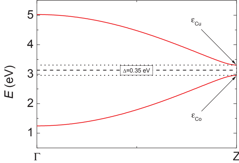
Figure 4.7: Band structure of the infinite variant of the DLCuCoW wire nanojunction over the first Brillouin zone. The band gap ( \Delta=0.35 eV) is marked by two dotted lines, between the copper ( \varepsilon_{Cu} ) and the cobalt ( \varepsilon_{Co} ) binding energies. The Fermi energy for the half-filled bands is represented by the dashed line.
