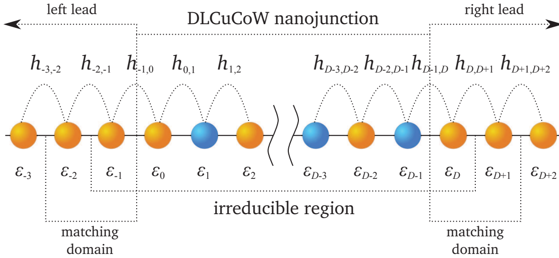
Figure 4.4: Schematic representations of the D -atomic linear nanojunction made of pairs of copper (orange color) and cobalt (blue color) atoms between copper leads. The corresponding binding energies \varepsilon_n for sites n , and the nearest-neighbor couplings h_{n,n'} between sites n and n' are depicted. Note that in order to keep the figures simple we show the nearest-neighbor coupling terms only for n < n' .
