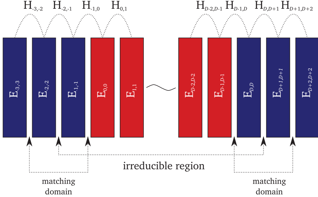
Figure 3.1: Schematic planar projection in the direction of propagation of an arbitrary three-dimensional Landauer-Büttiker-type system. The unit cells of the nanojunction ( N \in [0, D - 1] ) and two semi-infinite leads ( N \in [-\infty, -1] and N \in [D, \infty] ) are denoted by red and blue colors, respectively. The corresponding Hamiltonian on- and off-diagonal sub-matrices are also depicted. Note that in order to keep the figure simple we show the Hamiltonian sub-matrices for interactions between different unit cells only for i < j .
