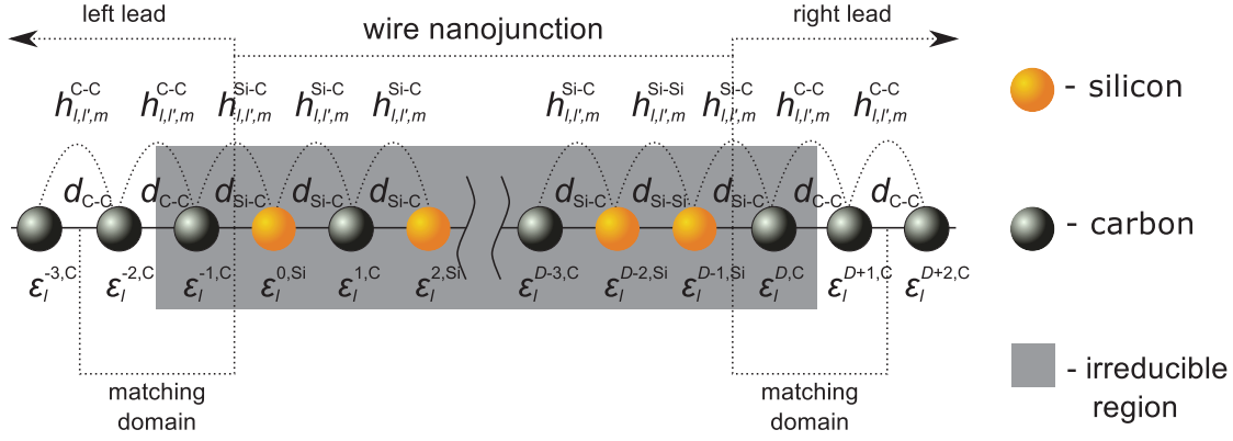
Figure 5.1: Schematic representation of the finite silicon-doped carbon wire nanojunction between two semi-infinite quasi one-dimensional carbon leads. The irreducible region and matching domains are distinguished (please see section 3.2 for more details). The binding energies for a given atomic site and the coupling terms between neighbor atoms with corresponding interatomic distances are depicted. The n and n' indices for the coupling parameters are dropped for simplicity.
