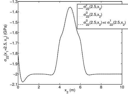
Figure 11: Example 2 ( \varepsilon = 0.01 m) – Stress \sigma_{22}(x_1 = 2.5, x_2) (GPa) on a vertical cut
