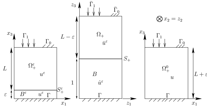
Figure 1: (a) Initial, (b) rescaled, and (c) limit configuration of a solid glued to a rigid base.
