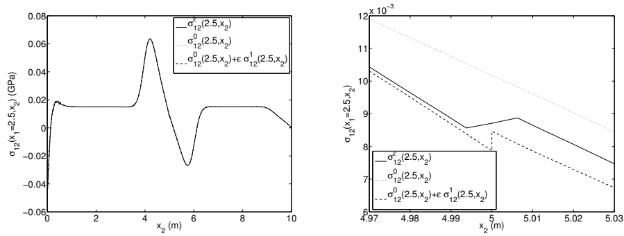
Figure 9: Exemple 2 ( \varepsilon = 0.01 m) – Stress \sigma_{12}(x_1 = 2.5, x_2) (GPa) on a vertical cut
