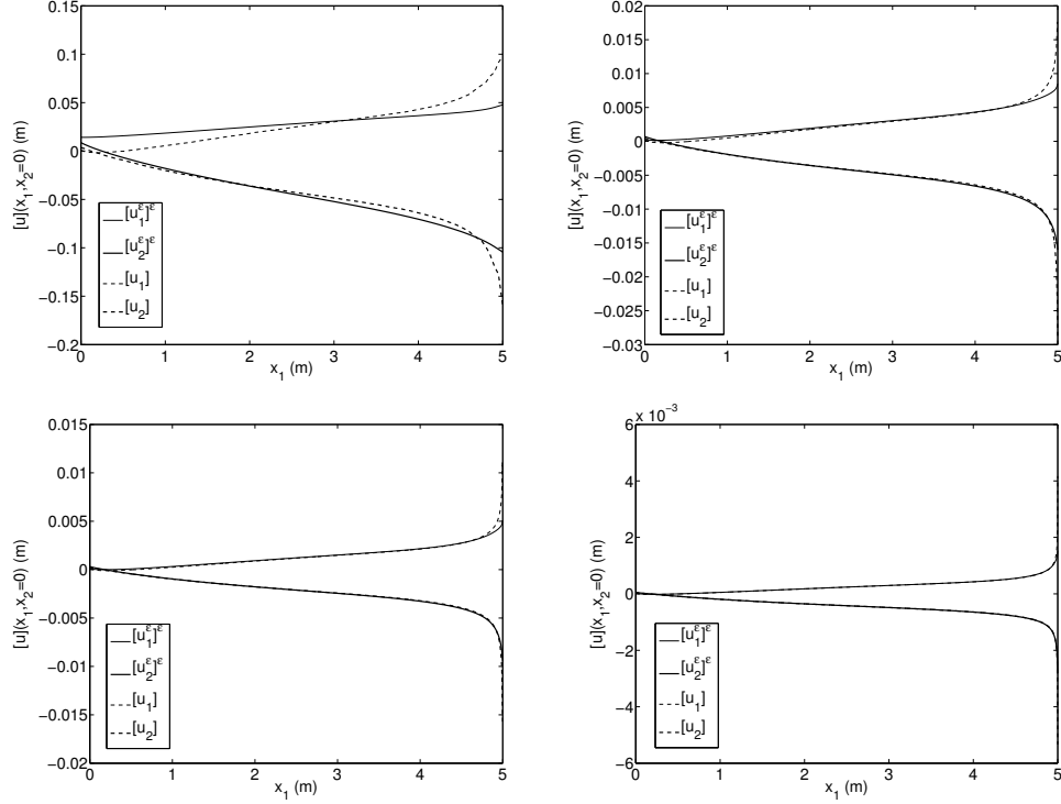
Figure 4: Exemple 1 – Jump in the displacement [u](x_1, x_2 = 0) (m) along the interface: \varepsilon = 0.1 m (left top), \varepsilon = 0.01 m (right top), \varepsilon = 0.005 m (left bottom) and \varepsilon = 0.001 m (right bottom)
