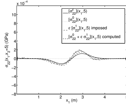
Figure 12: Example 2 ( \varepsilon = 0.01 m) – Jump in the stress [\sigma_{22}](x_1, x_2 = 5) (GPa) along the interface
