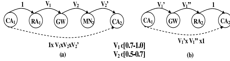
Fig. 3. Certificate Chain
