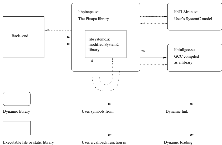
Figure 4.8: Link Mechanism in PINAPA
