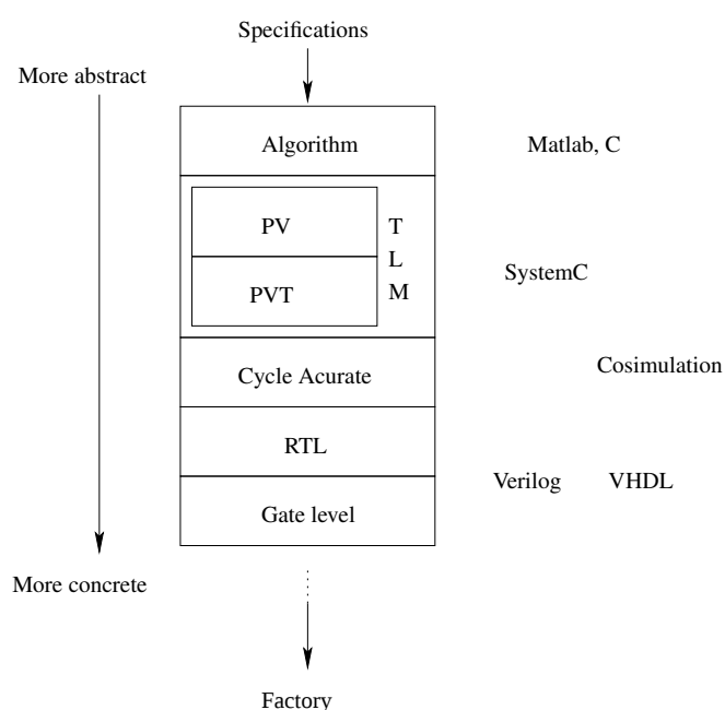
Figure 2.2: Illustration of the Different Levels of Abstractions
