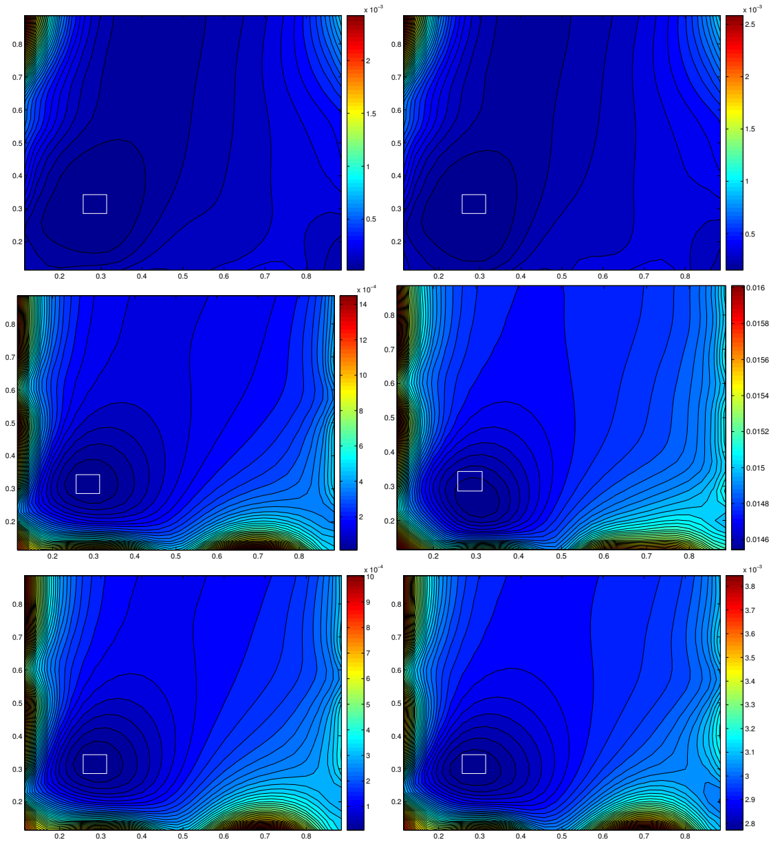
Figure 5. Contour maps of \mathcal{J}(\mathbf{C}) (top), \mathcal{H}(\mathbf{C}) with (A, B) = (50, 50) (middle) and \mathcal{H}(\mathbf{C}) with (A, B) = (1, 50) (bottom), plotted as functions of the location of the center of a trial four-element square defect. The graphs in the left and right columns correspond to no noise and a simulated relative noise of amplitude 1% on the synthetic data, respectively. The white square indicates the location of the “true” four-element defect.
